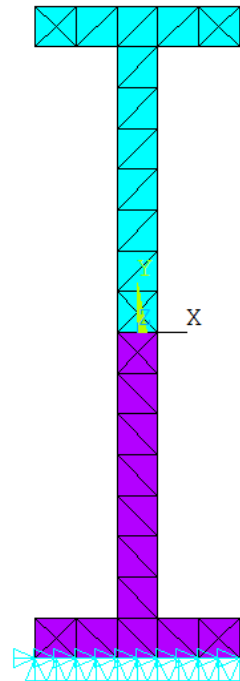
Fig. 2 Finite element model with boundary conditions for modal analysis with different materials shown
