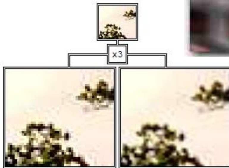
Bilinear Interpolation
