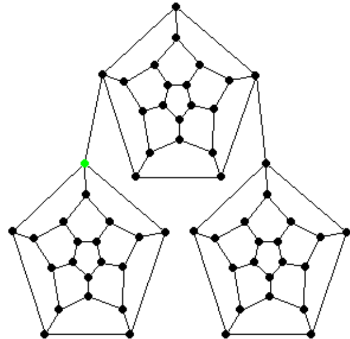
Breadth-First Search
