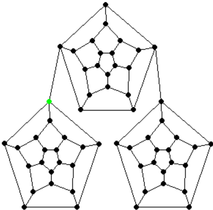
Depth-First Search
