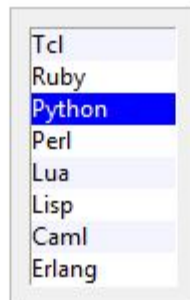
Listbox widgets.
