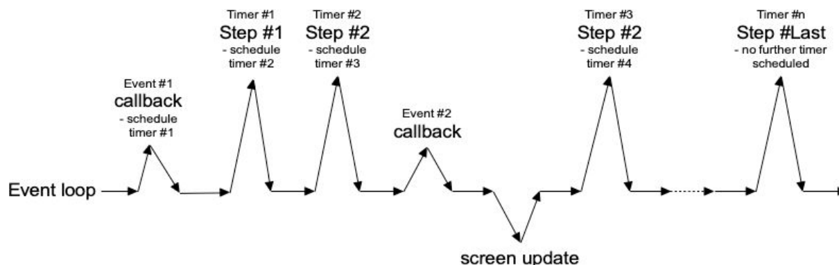
Breaking up a large operation into small steps tied together with timer events.
