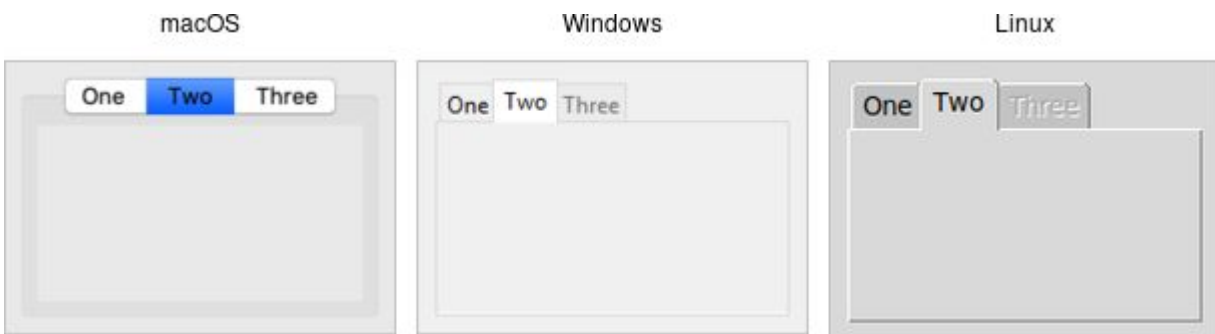
Notebook widgets.
