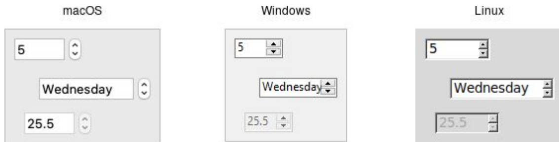
Spinbox widgets.
