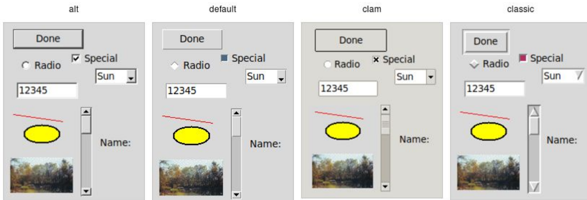
Built-in themes.
