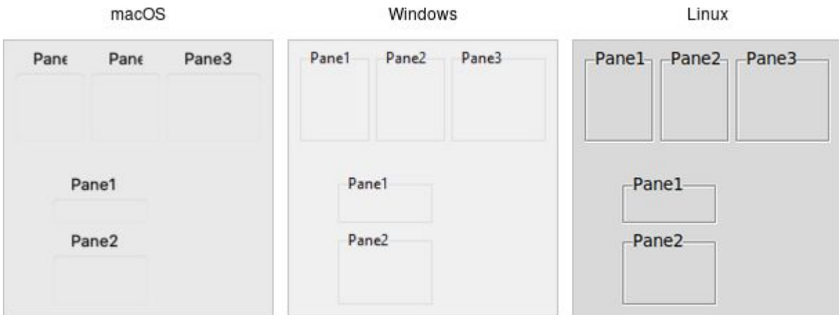
Panedwindow widgets (shown here managing several labelframes).
