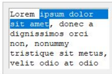
Text widgets.
