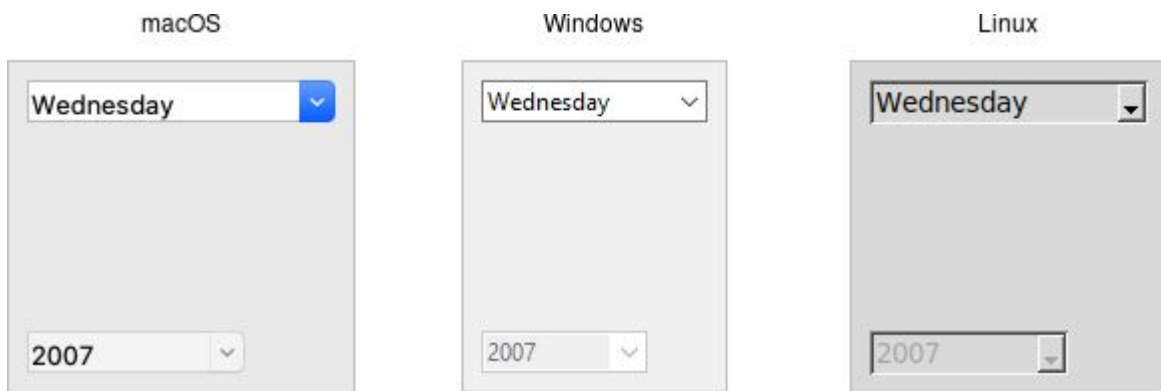
Combobox widgets.
