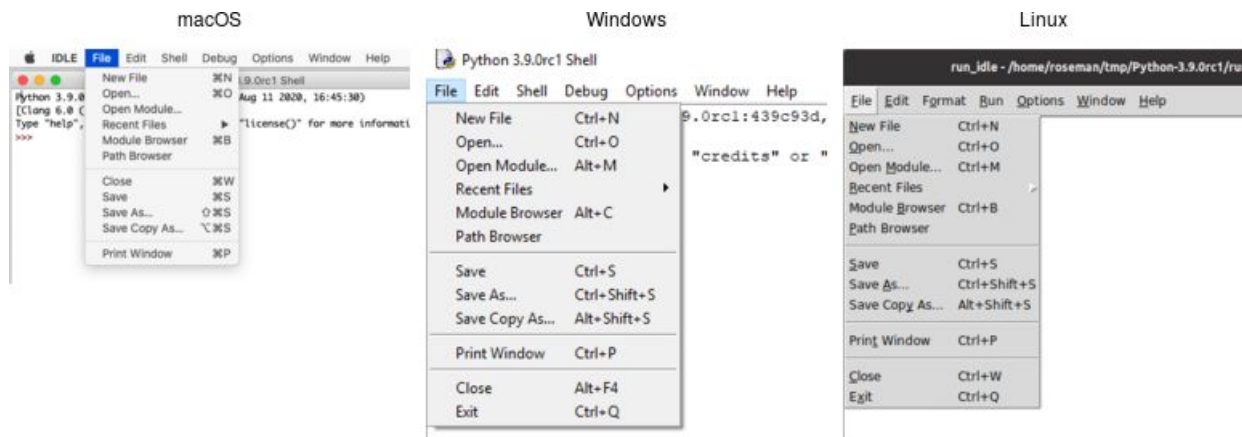
Menubars.
