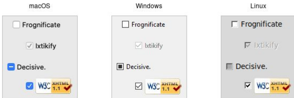
Checkbutton widgets.
