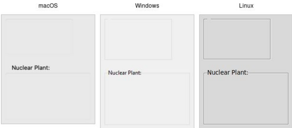
Labelframe widgets.
