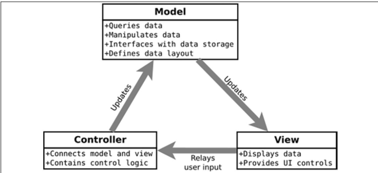
Figure 6.1: The roles and relationships of Model, View, and Controller Let's take a deeper look at each of these components and understand them in the context of our current application.
