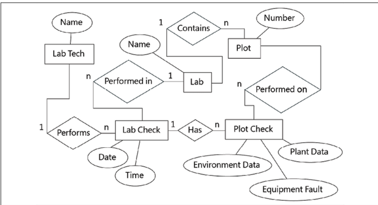
Figure 12.1: An entity-relationship diagram of our ABQ data
