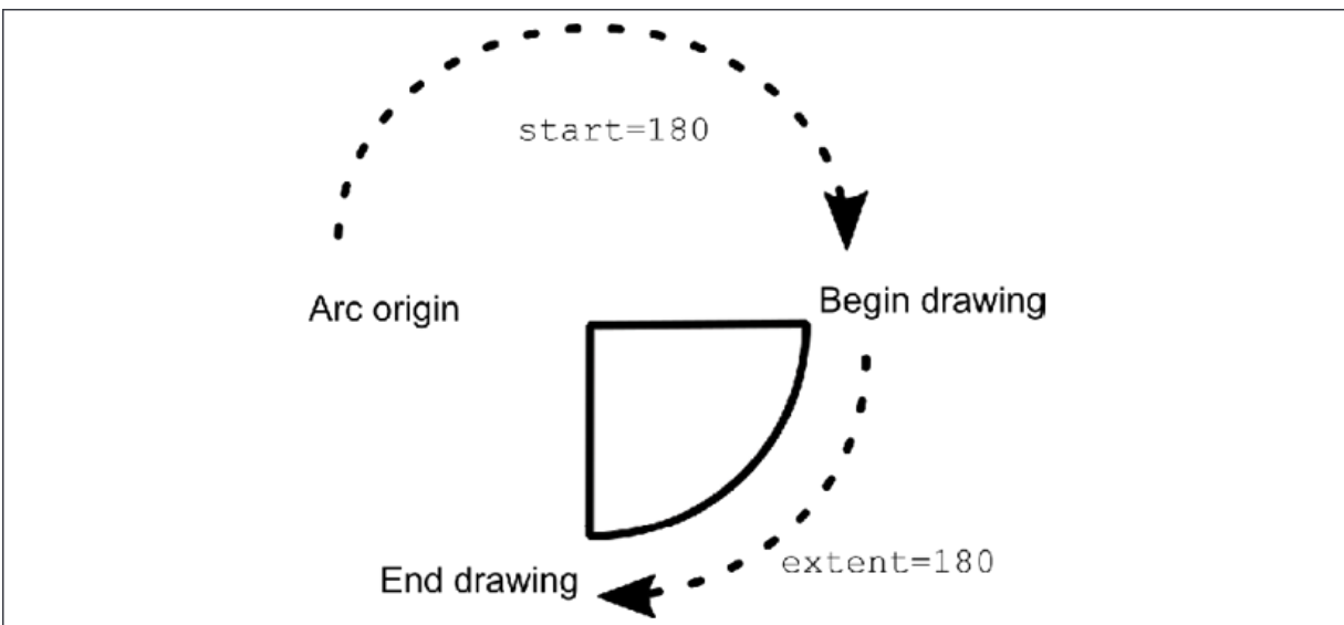
Figure 15.1: Drawing an arc Let's add an arc to our demo:
