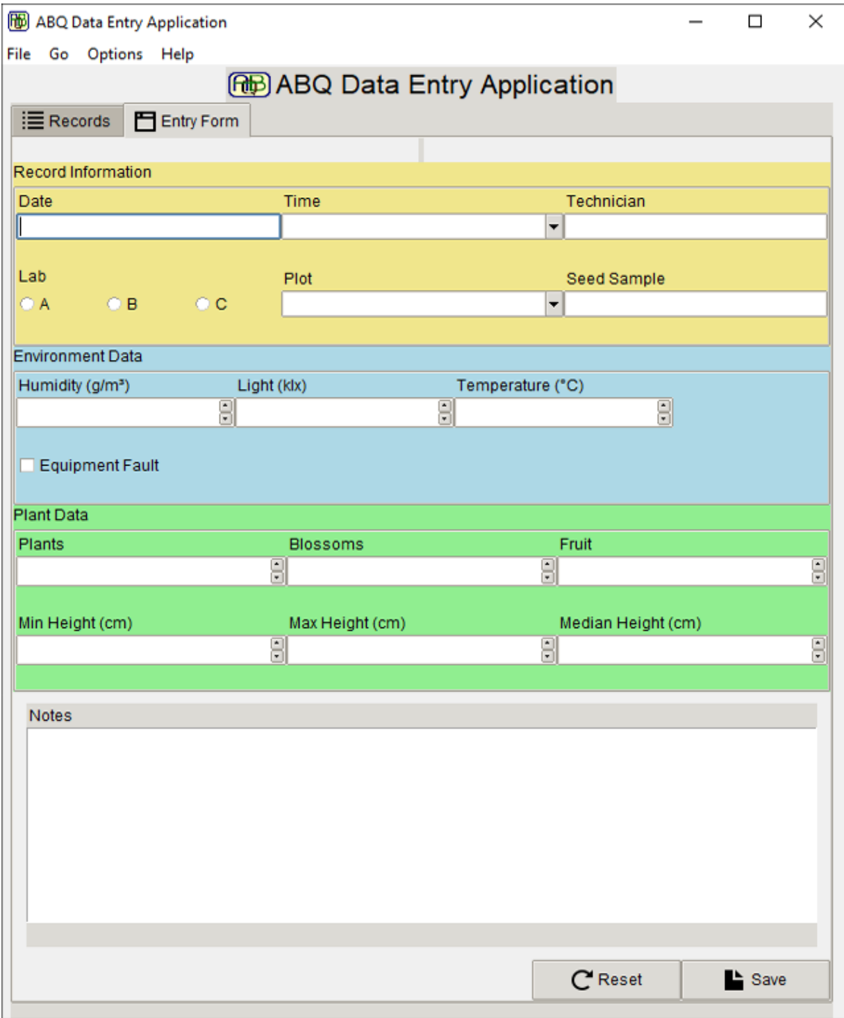
Figure 9.17: ABQ Data Entry using the "clam" theme on Windows As you can see, not every theme looks so good with our changes. Try the different themes available on your platform. Which theme looks best on your platform? Which ones work best with our style changes? Try them all out and see.
