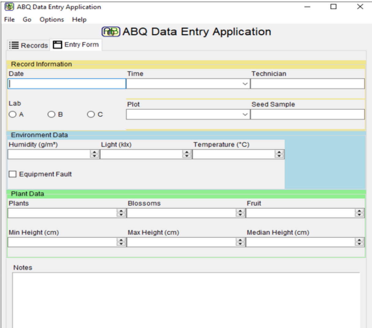
Figure 9.14: Our first attempt at coloring our record form frames As you can see, that's far from ideal. While there is a small amount of color peeking out from behind the widgets, the widgets in each section are still the default drab color, and even the label portion of the LabelFrame widgets is still gray. Styles do not propagate to child widgets, so we're going to have to set each widget individually to get the full effect.
