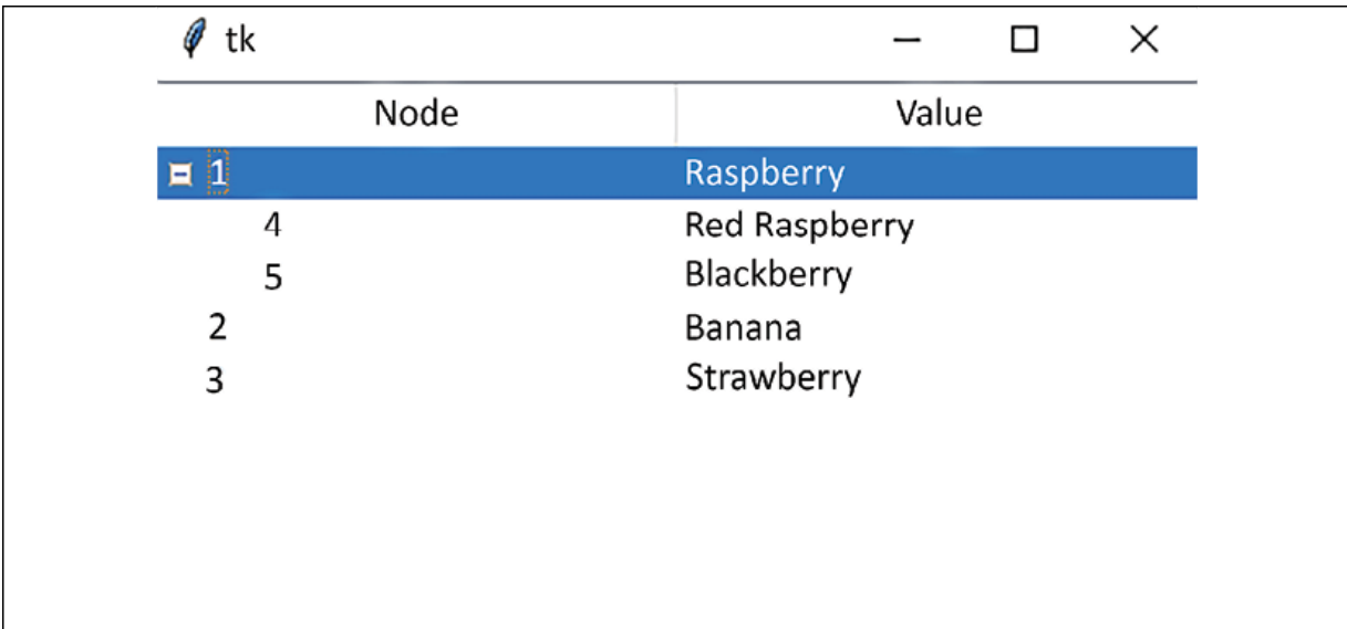
Figure 8.2: The berry hierarchy displayed in a Treeview widget. Each item in a treeview is identified by a unique item identifier (IID) , and each column by a column identifier (CID) . These values are strings, and you can either assign them manually or let the widget choose them automatically.
