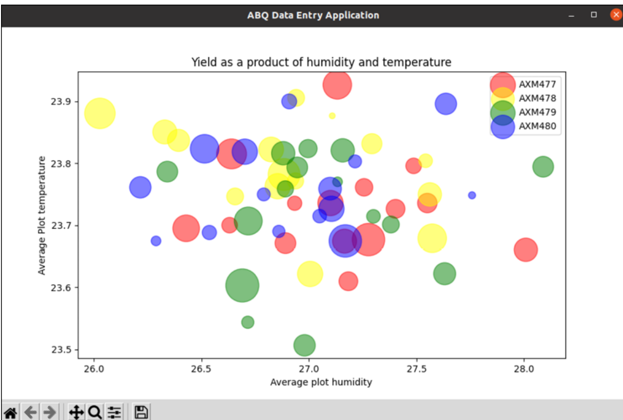
Figure 15.5: Our scatter plot showing how seed samples performed under different conditions. Take a moment to play with this chart using the navigation toolbar. Notice how you can zoom and pan, adjust the size of the chart, and save the image. These powerful tools are provided by Matplotlib automatically, and make for very professional-looking charts.
