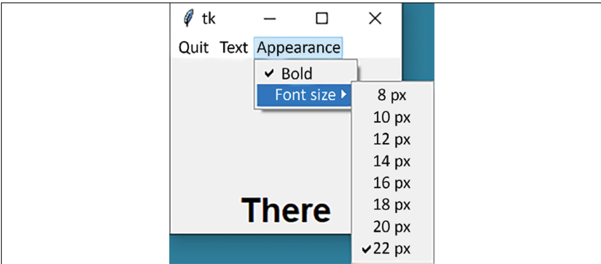
Figure 7.10: The Menu demo application
