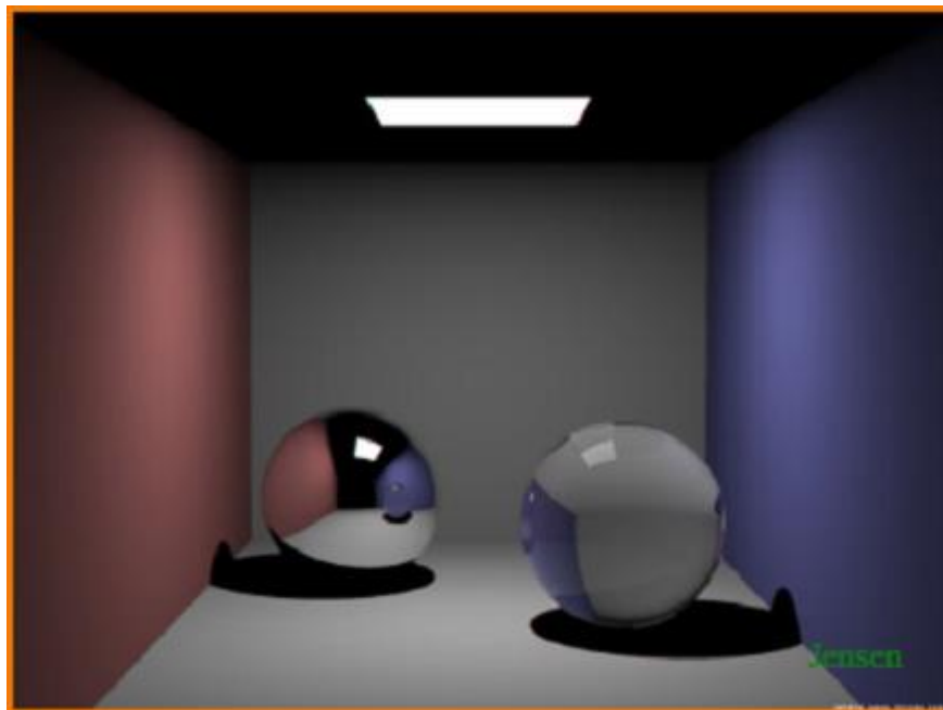
Ray Tracing
