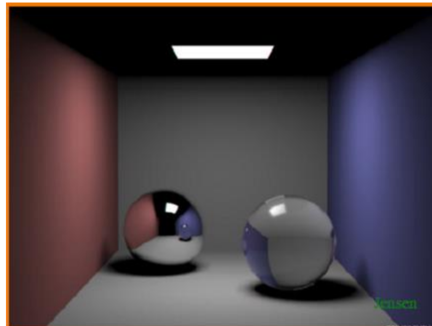
+ soft shadows
